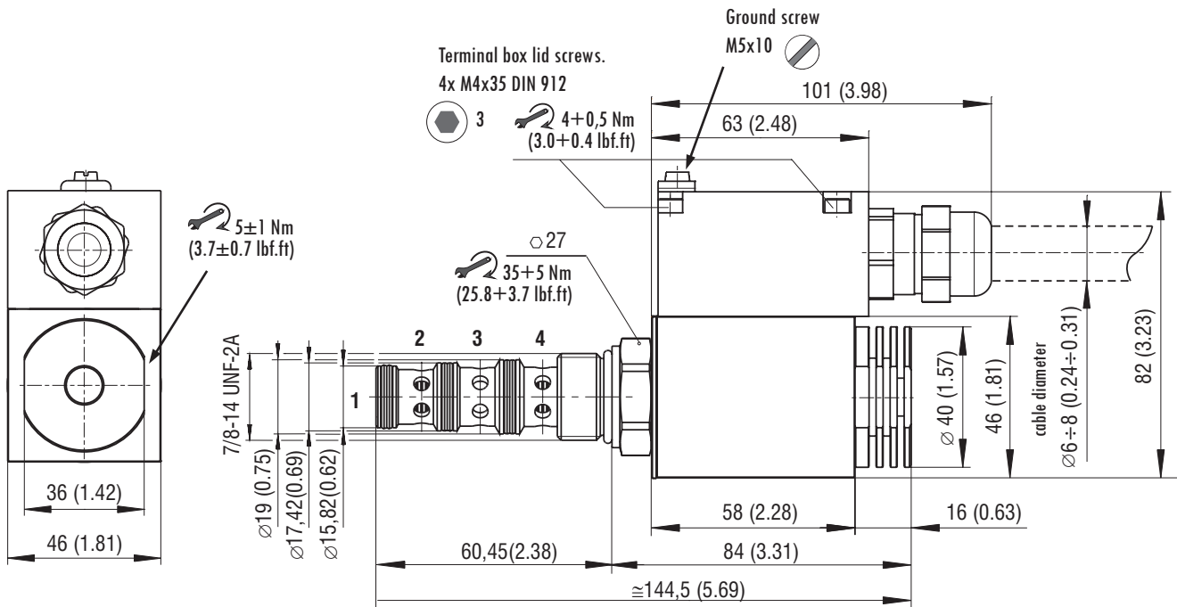
Dimensions of SD2PX-B4 valve, dimensions in mm (in)
