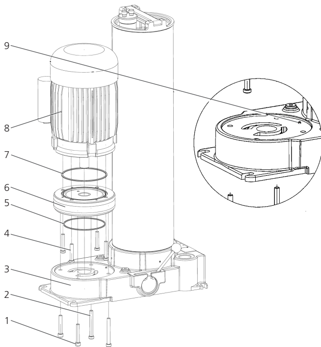
Fig. 8: Replacing the motor and the pump
