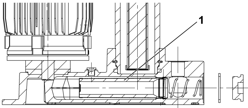
Fig. 10: Installing the suction filter element
