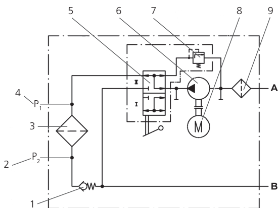
Fig. 12: Hydraulic circuit diagram
