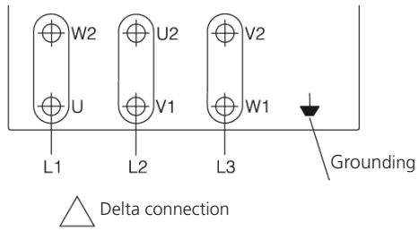
Fig. 13: Connection plan
