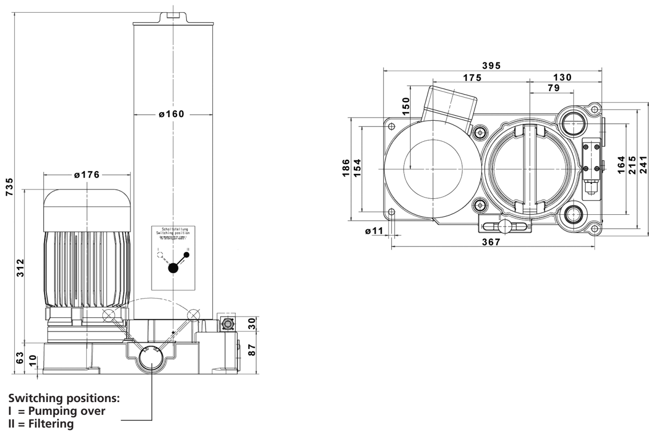
Fig. 11: Device dimensions
