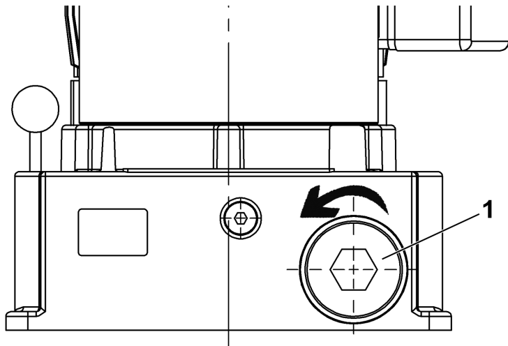
Fig. 9: Removing the suction filter element
