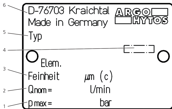
Fig. 2: Nameplate
