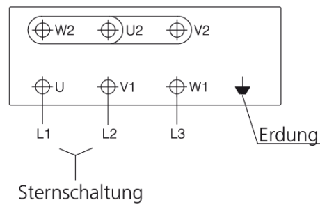
Anschlüsse
