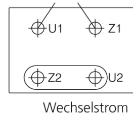
Anschlüsse
