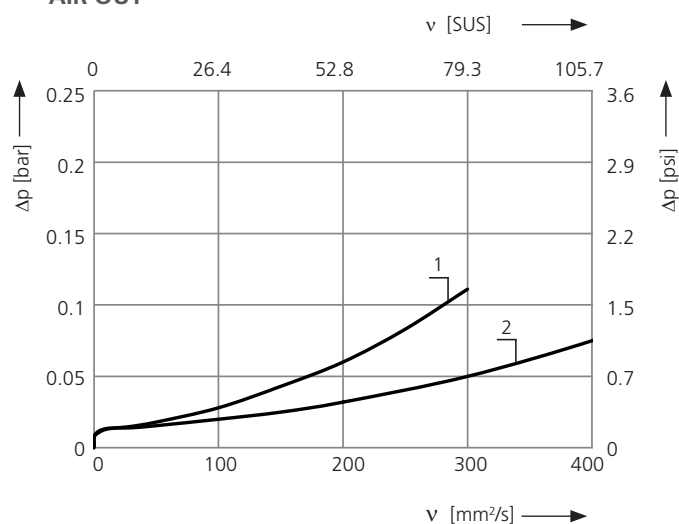
Pressure drop as a function of the flow volume AIR OUT
